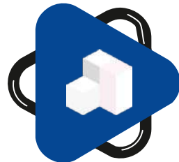
3D Segmentation
